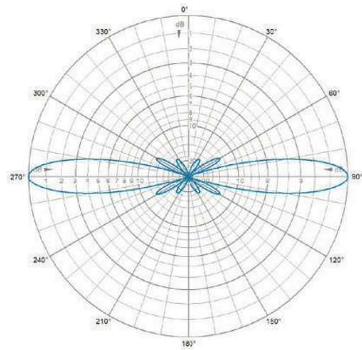
E-Plane | 875 MHz
