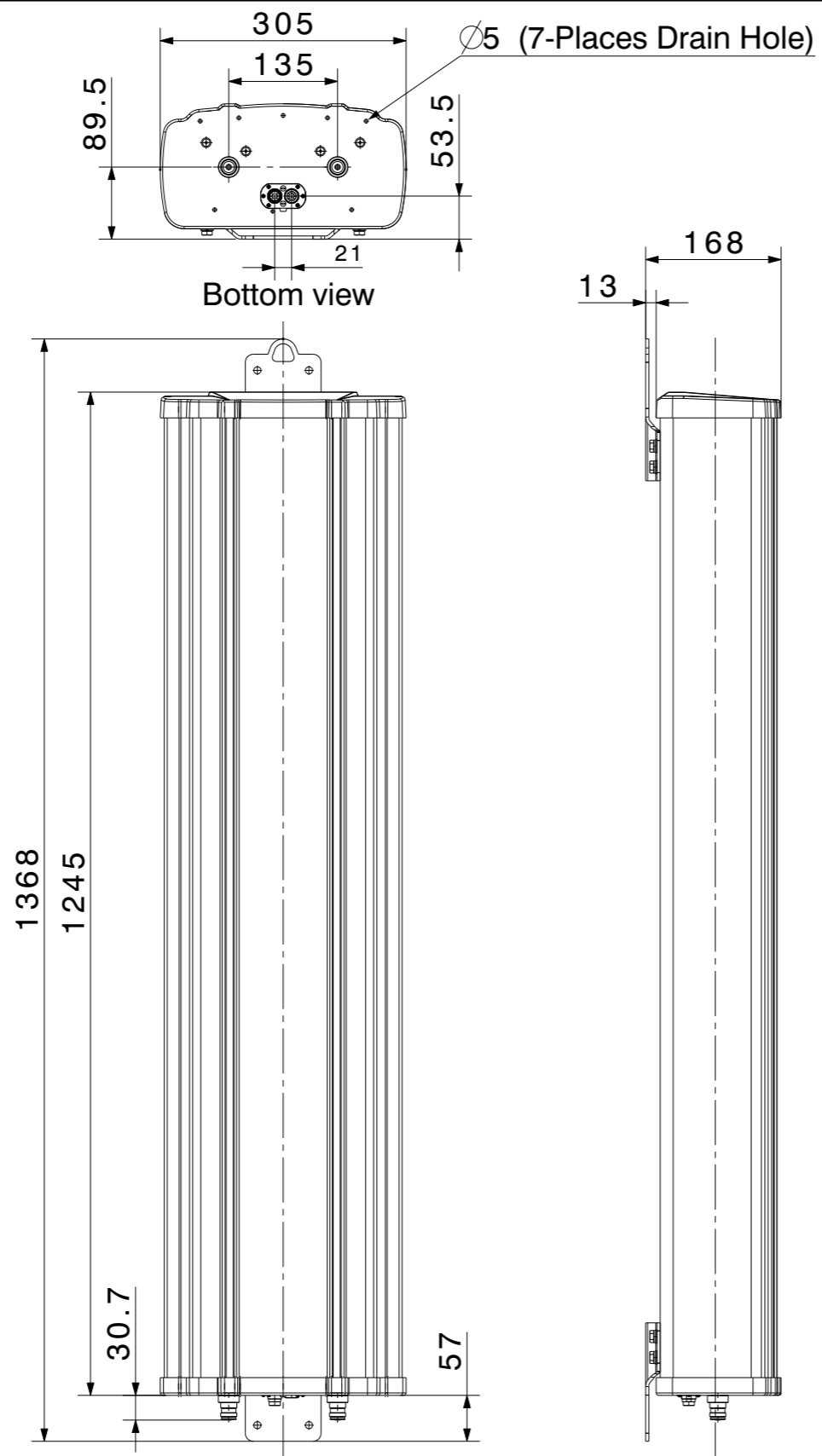
Front view
