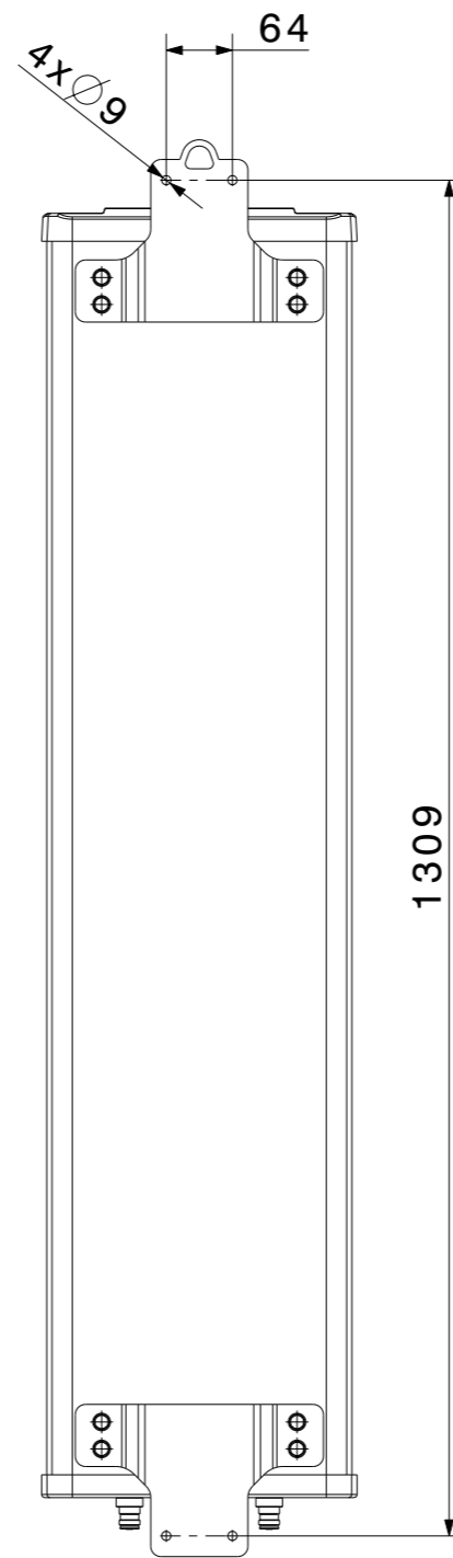
Rear view
