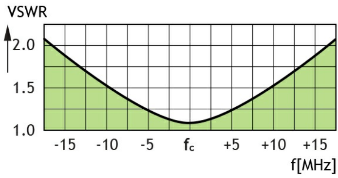
TYPICAL VSWR CURVE
