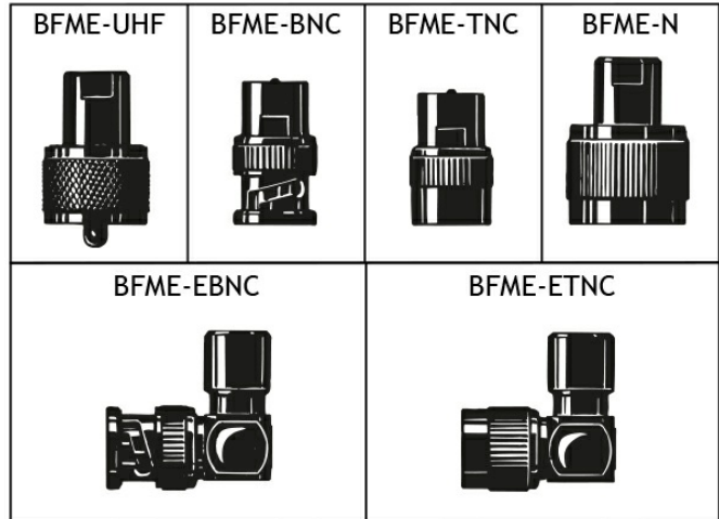
RECOMMENDED BFME-CONNECTORS
