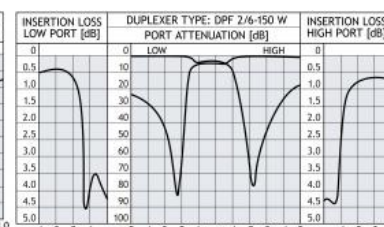
TYPICAL RESPONSE CURVES @ 4.5 MHz DUPLEX SPACING
