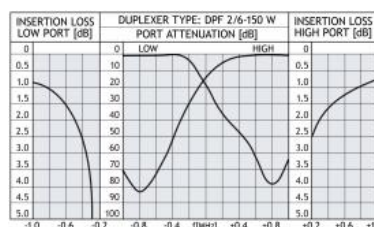
TYPICAL RESPONSE CURVES @ 1.6 MHz DUPLEX SPACING
