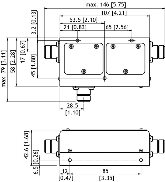
Mounting Details for PRO-IS-150-D1
