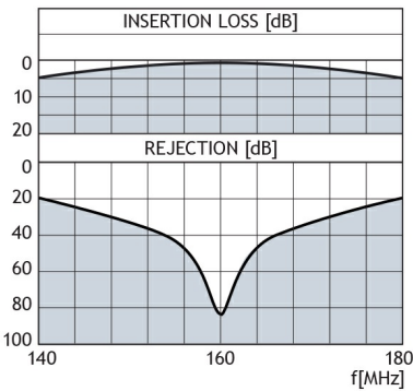
Typical response curves for PRO-IS-150-D1
