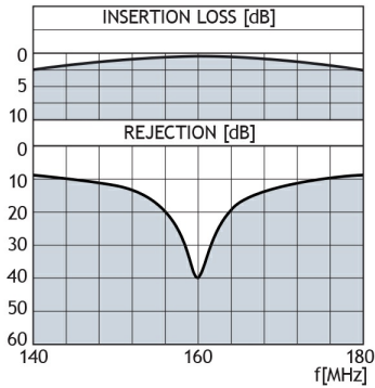
Typical response curves for PRO-IS-150-S1
