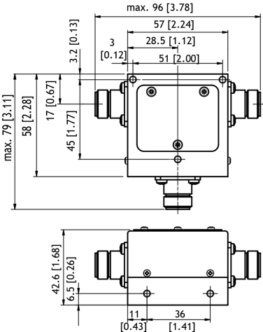
Mounting Details for PRO-IS-150-S1
