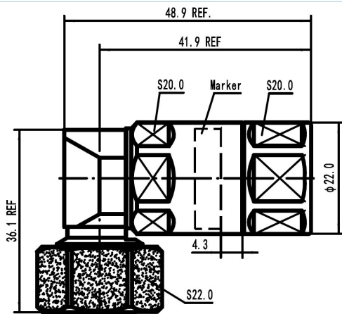
43MR-LCF12-C03 Outline drawing
