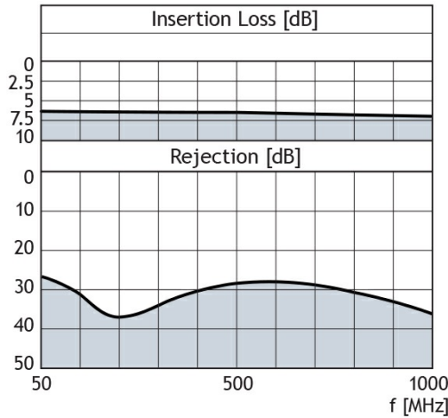
INSERTION LOSS & ISOLATION
