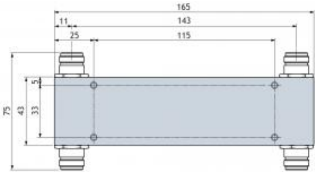
Mounting Details
