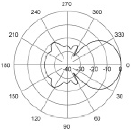
E-Plane | 405 MHz
