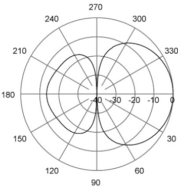
E-Plane | 82 MHz
