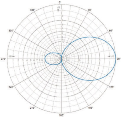
E-Plane | 405 MHz
