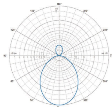
E-Plane | 405 MHz
