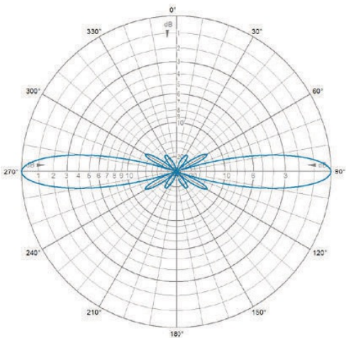
E-Plane | 405 MHz
